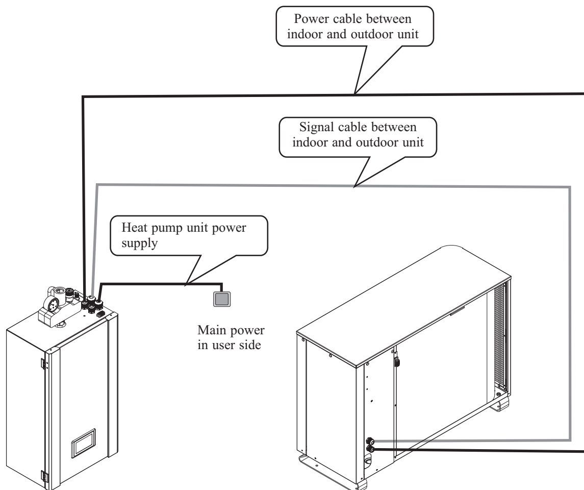
Installation sketch
